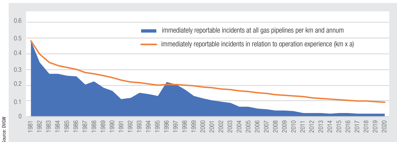
Figure 9: Development of Immediately Reportable Incidents at All Gas Pipelines Throughout the Years 1981 to 2020
